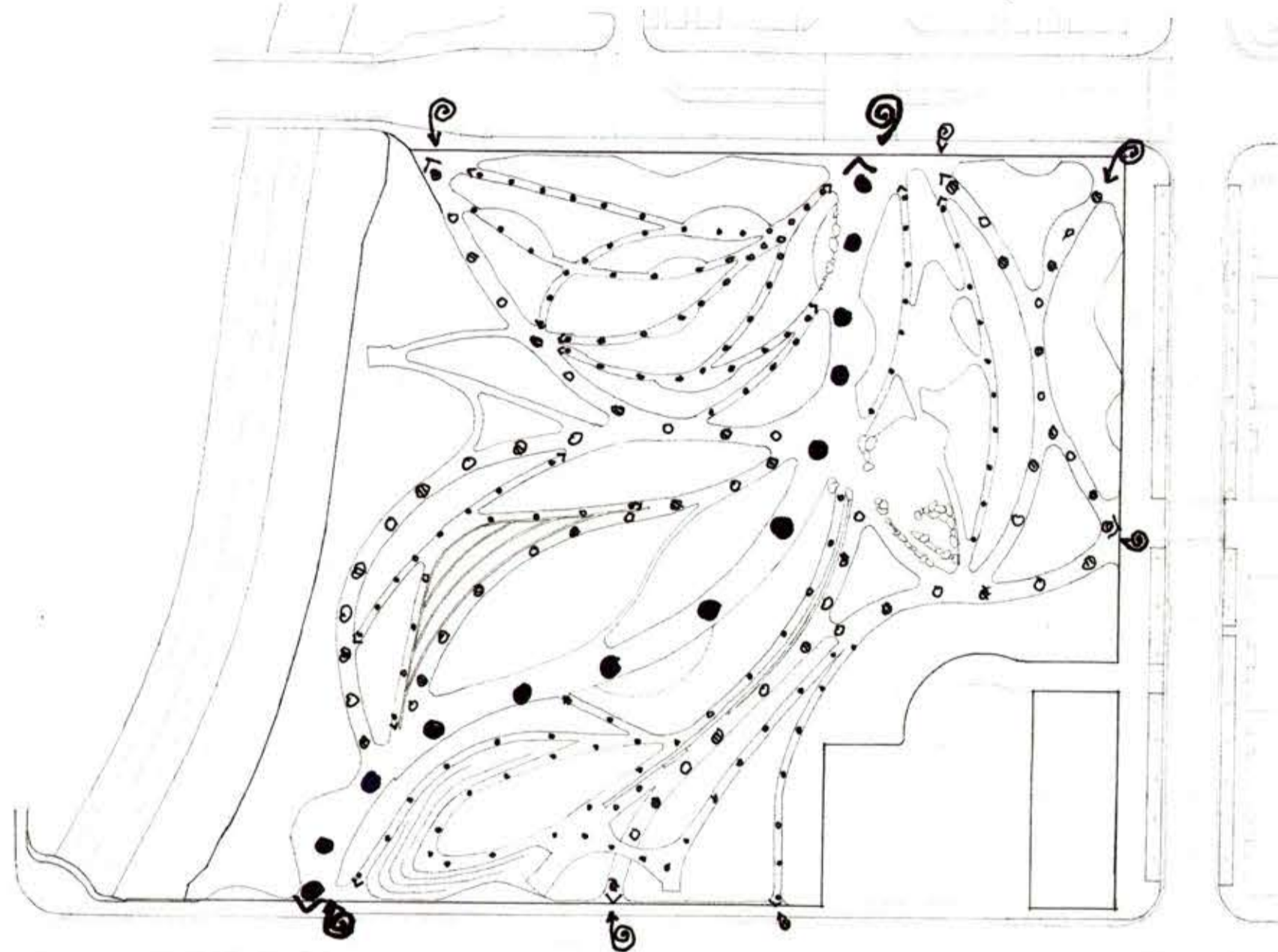
PEDESTRIAN CIRCULATION
